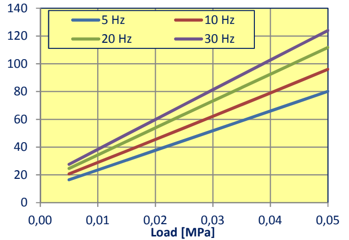
Dynamic bedding modulus (MN/m 3 )(3)
